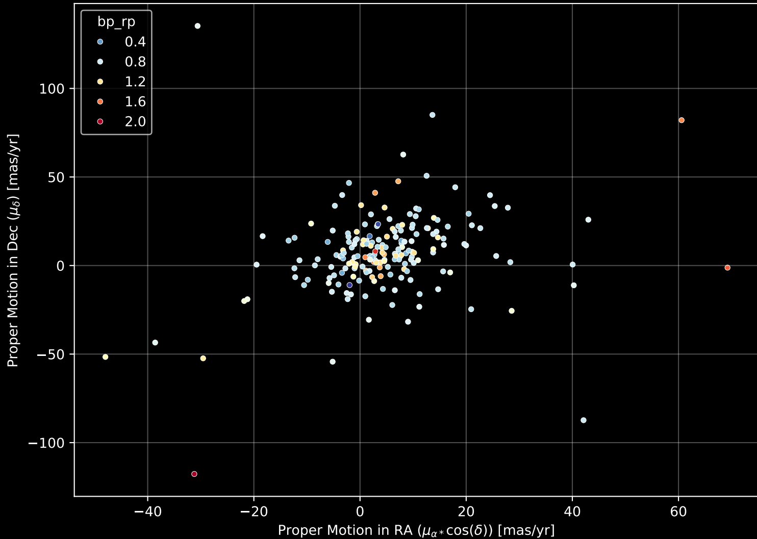
GALAH DR4 Field: [7157] Proper Motion Diagram (n= 195)
