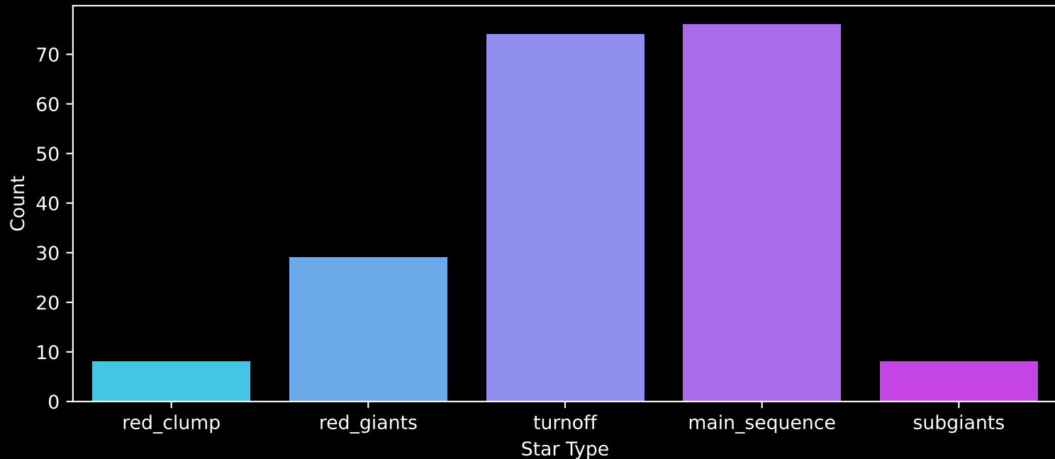
GALAH DR4 Field: [7157] Count plot of Star Type
