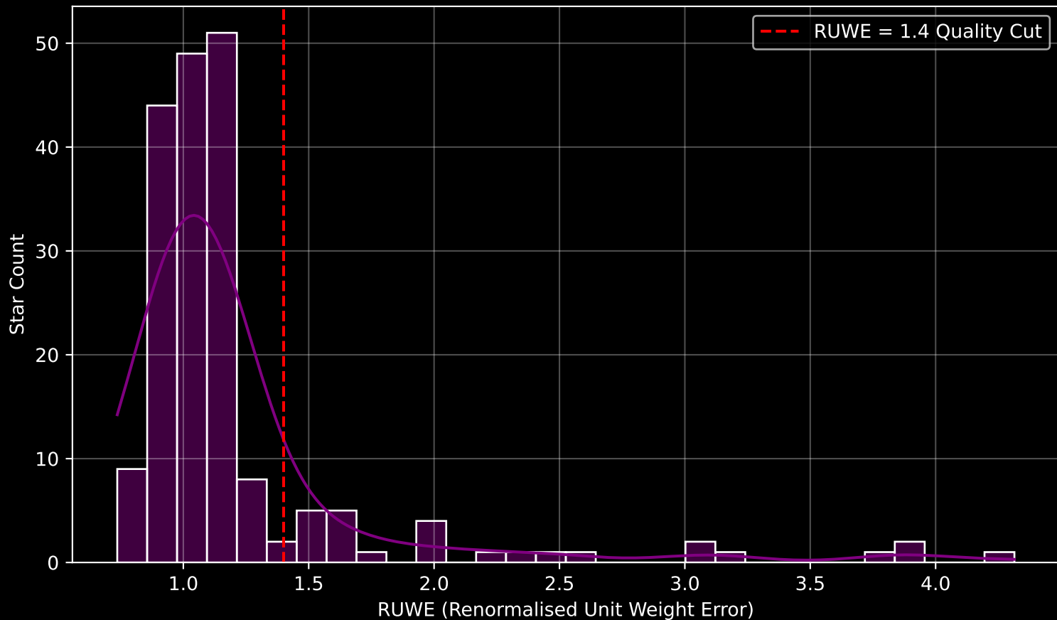
GALAH DR4 Field [7157] RUWE Distribution (n= 189)
